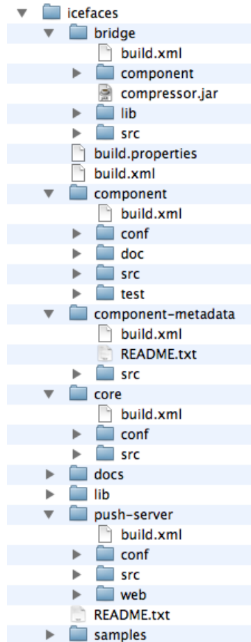
Figure 3 ICEfaces Source Distribution Directory Structure
