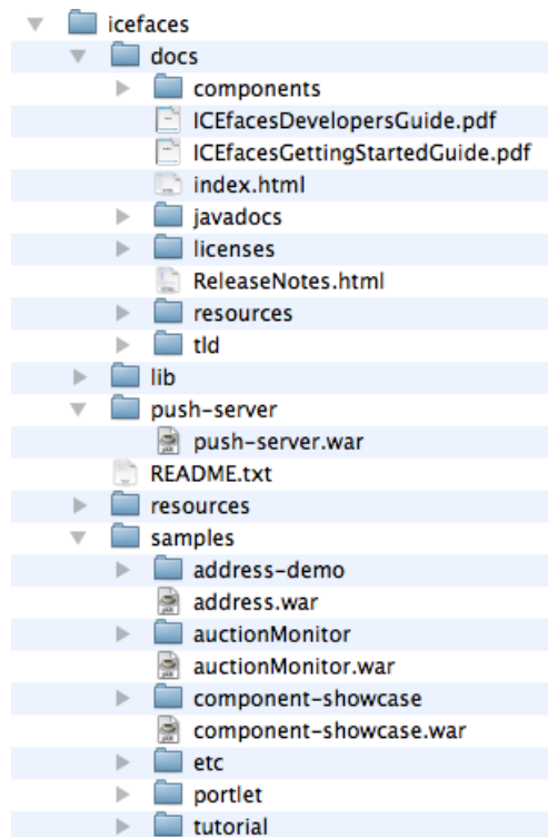
Figure 2 ICEfaces Directory Structure
